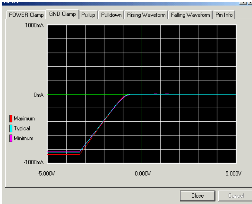
Figure 4 • Sample GND Clamp Curve
