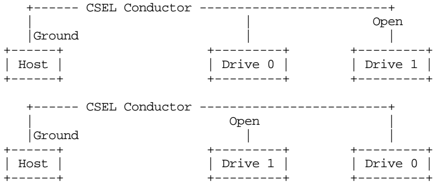
Figure 5 - Cable select
