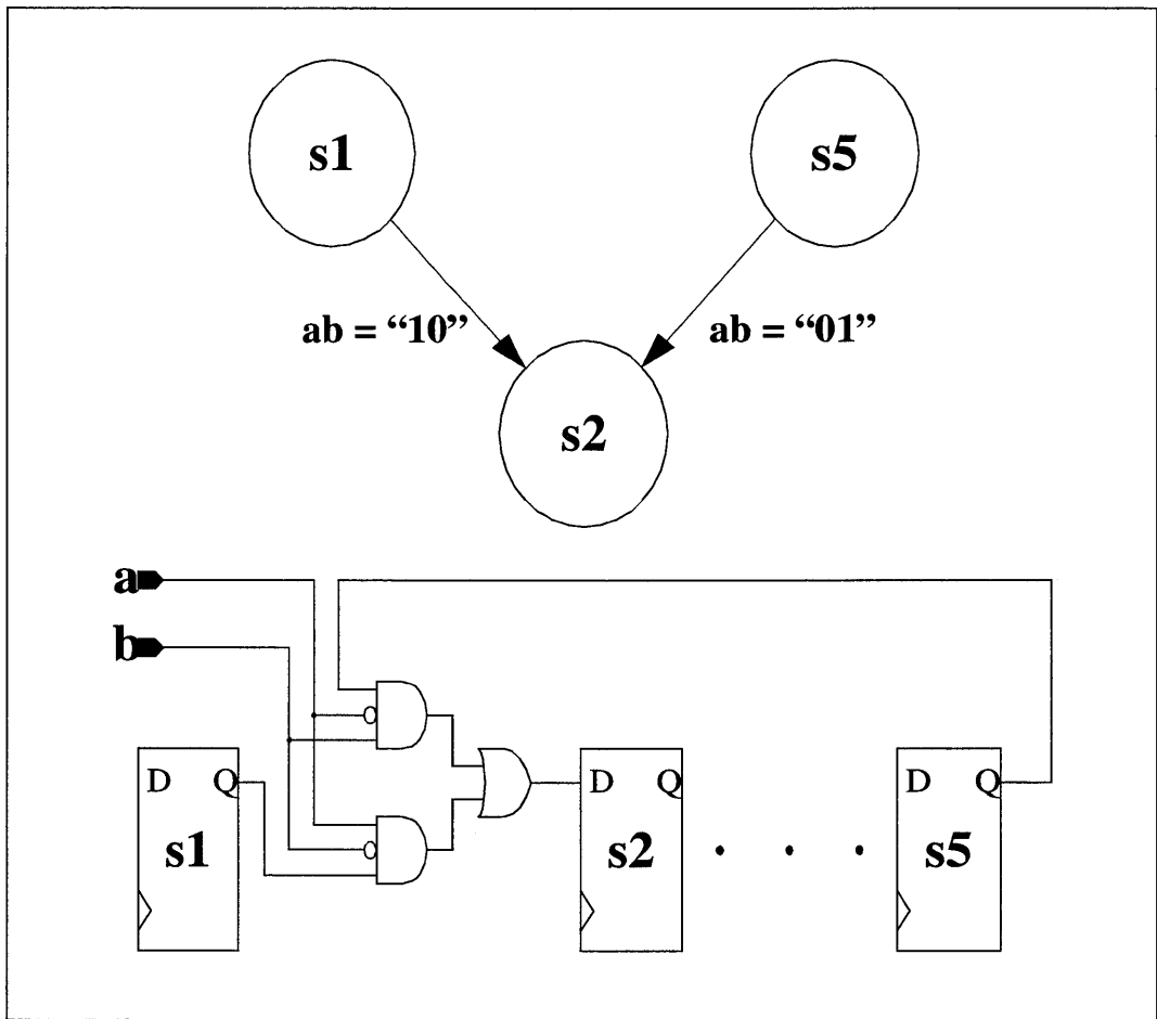
Figure 4-9. Implementation of one-hot state machine bits
