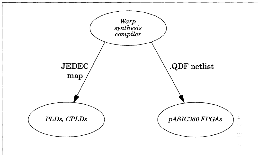
Figure 1-1. The Warp synthesis compiler produces JEDEC maps for programming PLDs and CPLDs, and .QDF netlists for placing and routing pASIC380 FPGAs.
