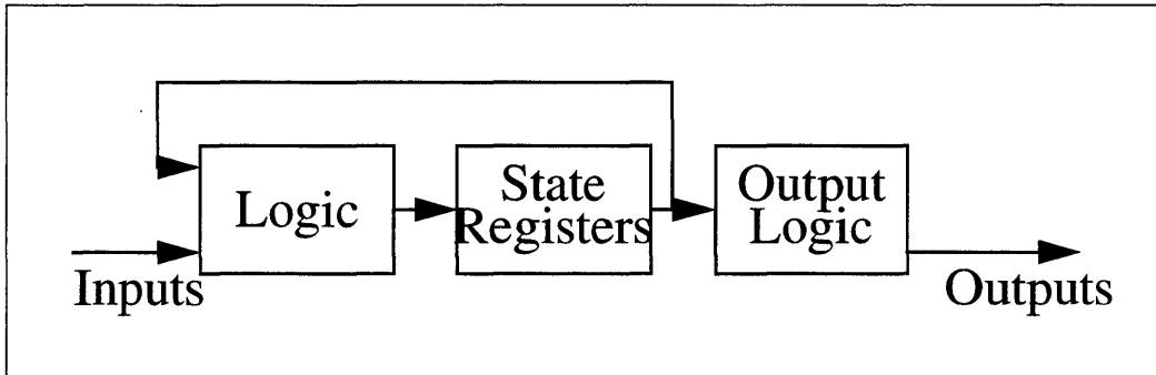
Figure 4-5. Outputs Decoded Combinatorially
