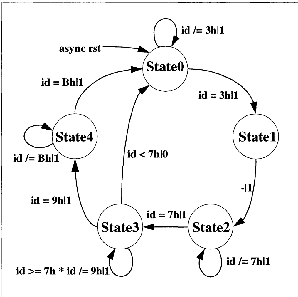
Figure 4-10. State Diagram for Combination Moore-Mealy State Machine
