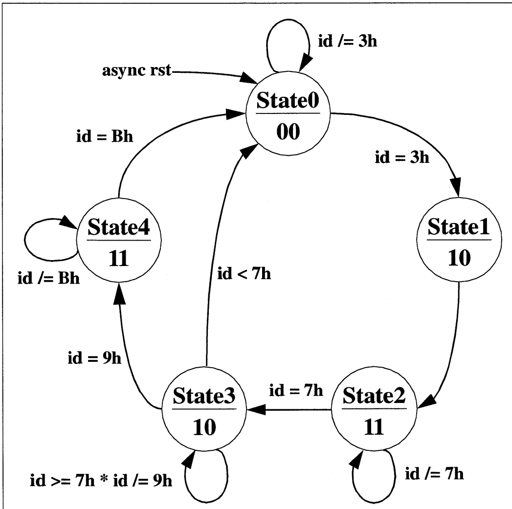
Figure 4-4. State Diagram of Moore State Machine
