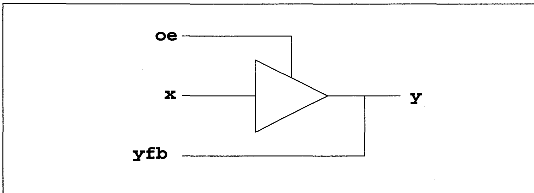
Figure 4-3. Bufoe Component.
