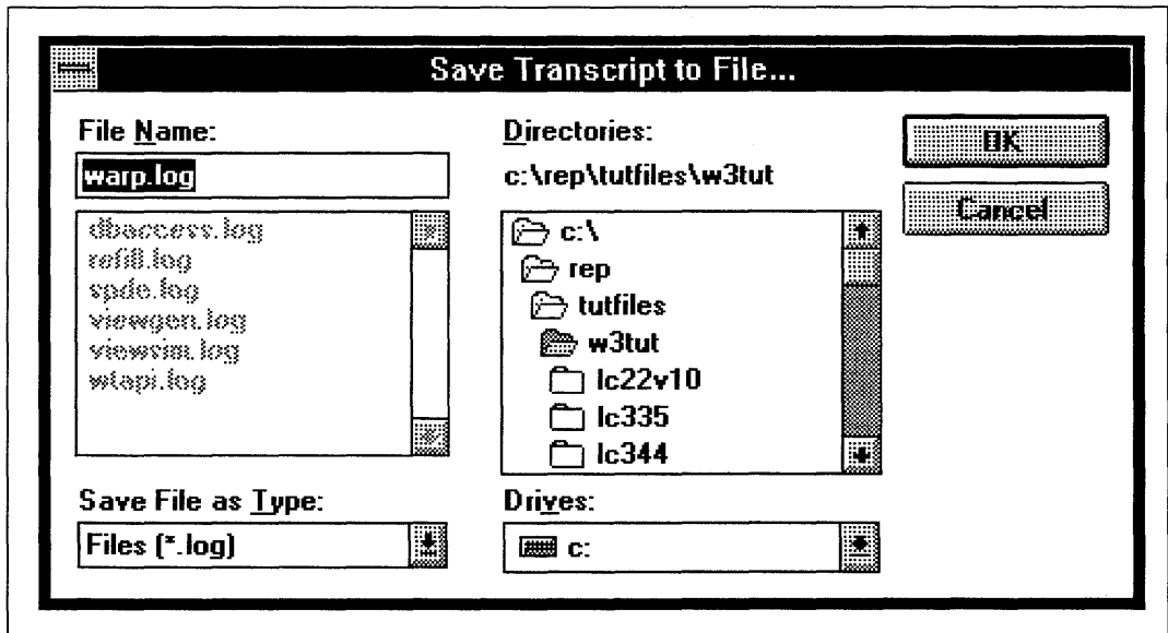
Figure 3-4. Save Transcript to File... Dialog Box.
