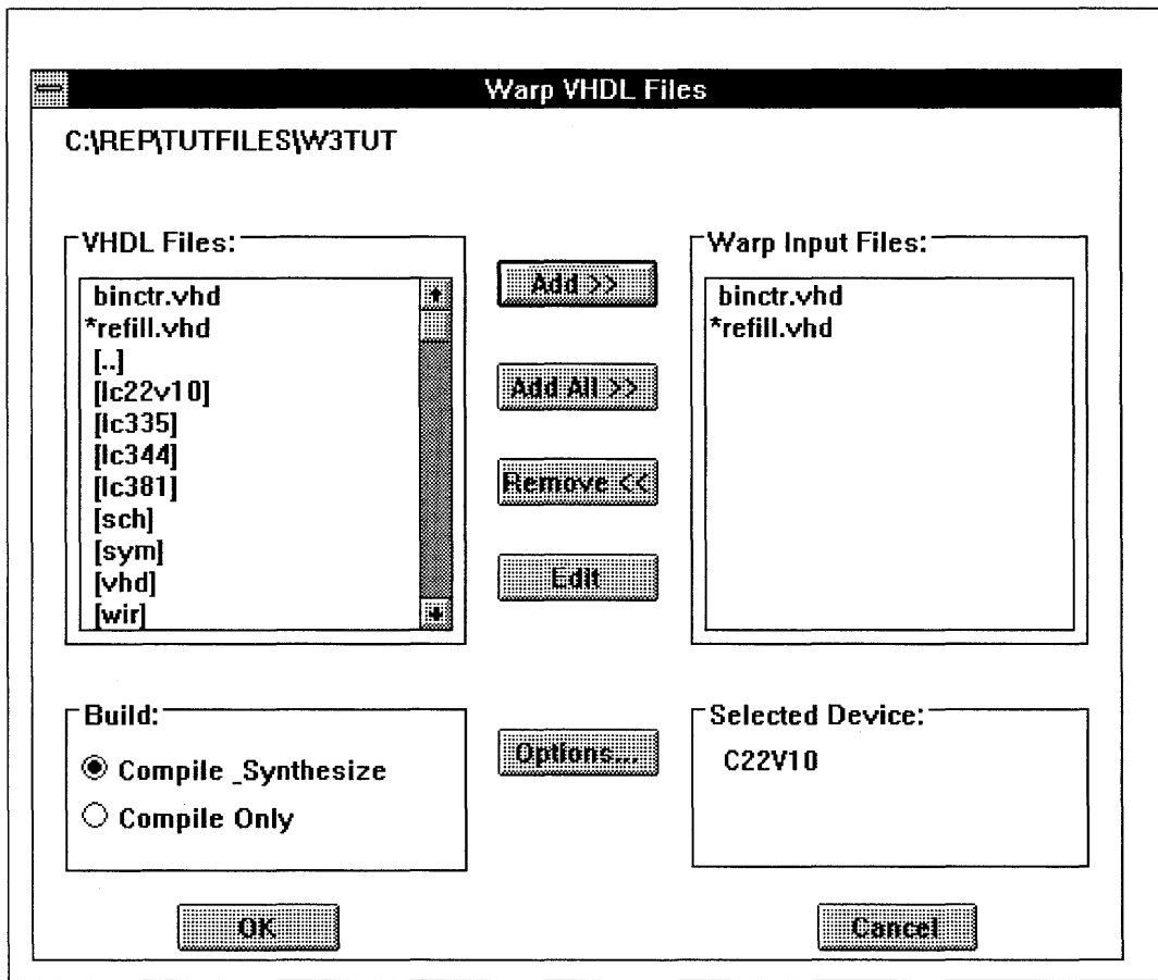
Figure 3-11. Warp VHDL Files Dialog Box.
