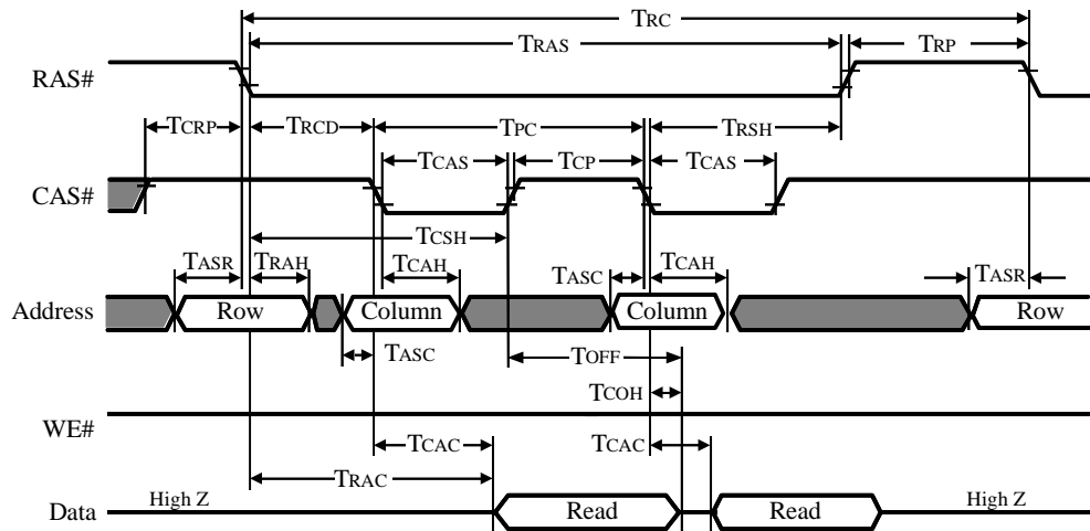
Figure 16-7: DRAM Read Cycle Timing
