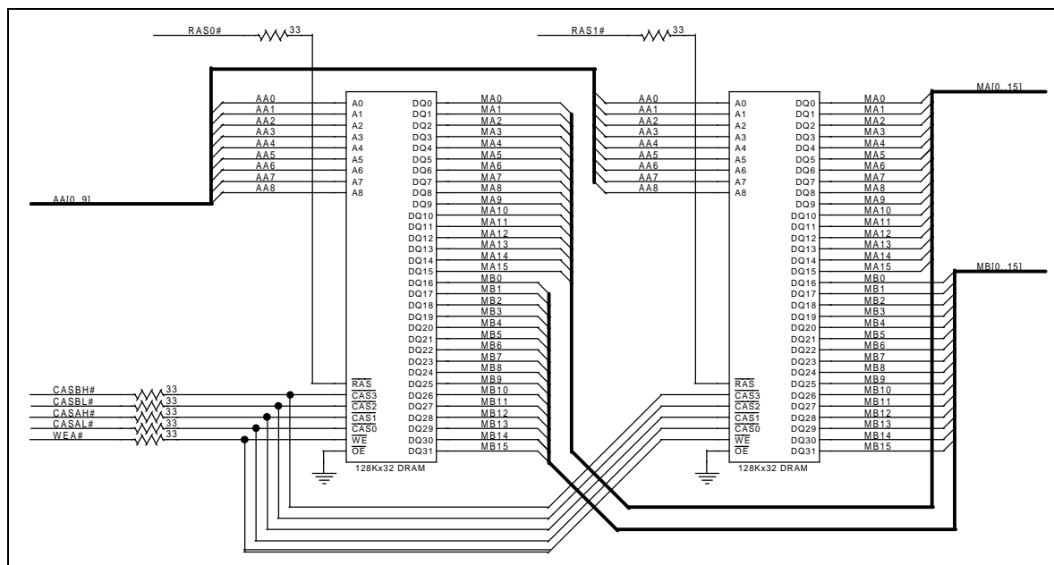
Figure F-2: 1MB, 32-bit Memory Configuration Using Two 128Kx32 DRAMs
