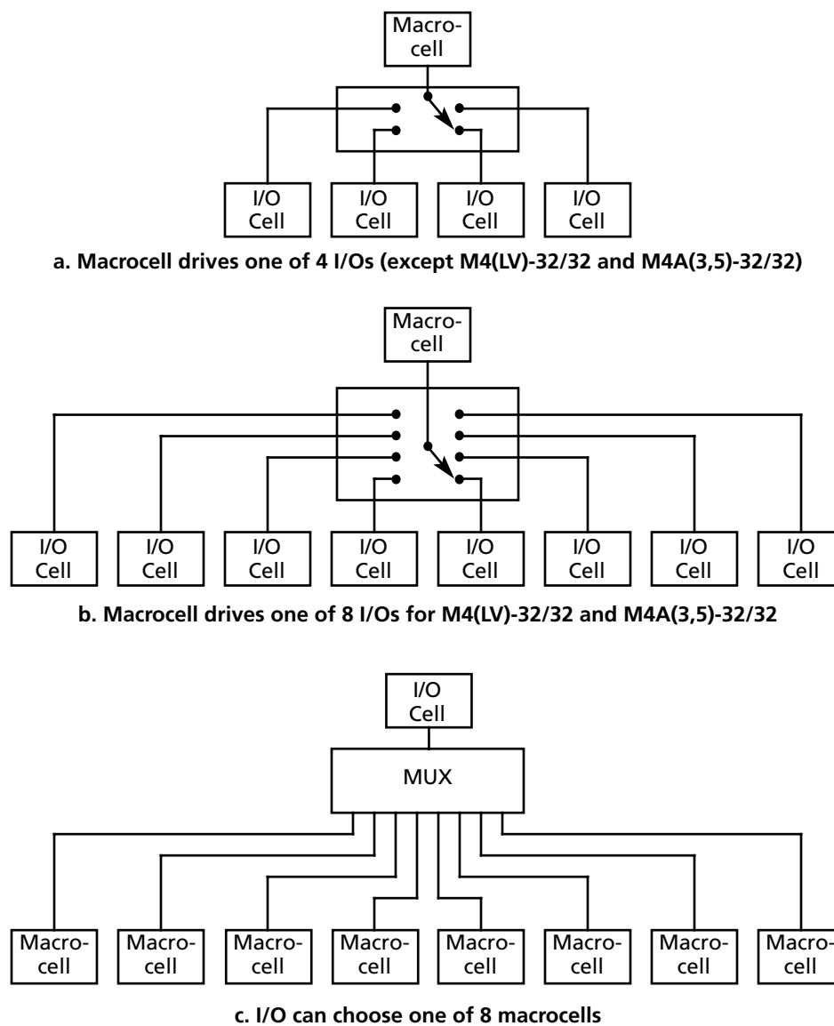
Figure 9. MACH 4 Output Switch Matrix
