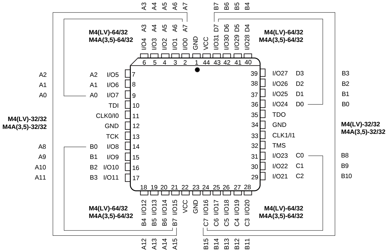
44-Pin PLCC
