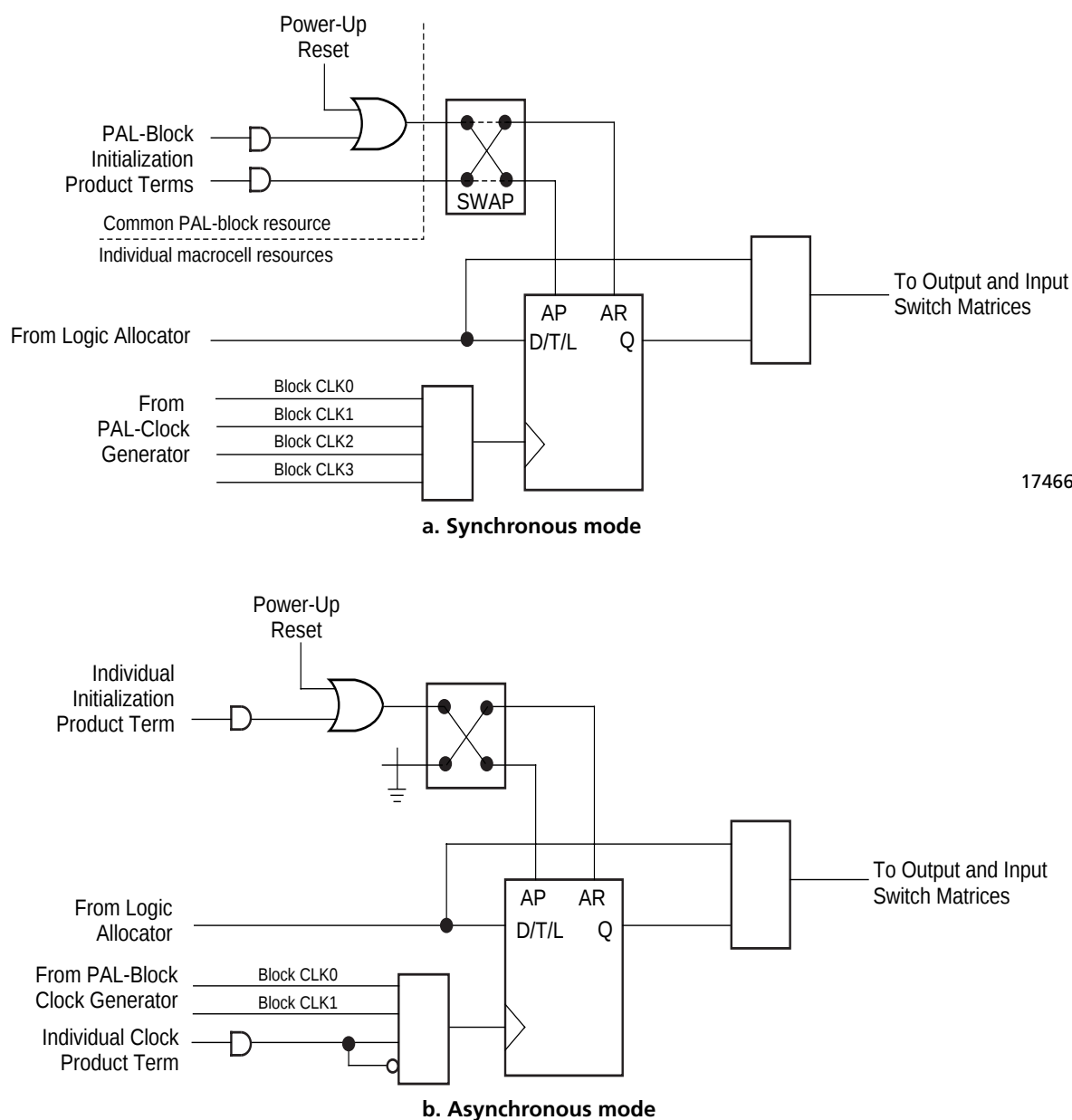
Figure 5. Macrocell
