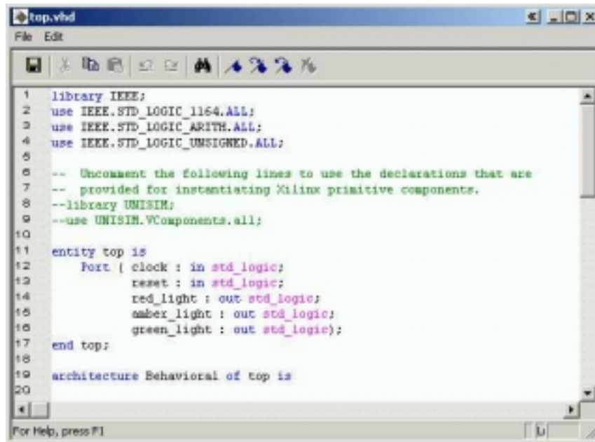
Figure 4.5.4 New VHDL File
