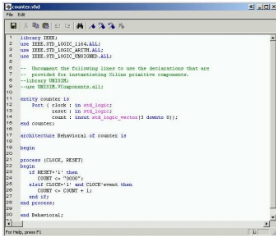
Figure 4.2.5 Counter in VHDL Window
