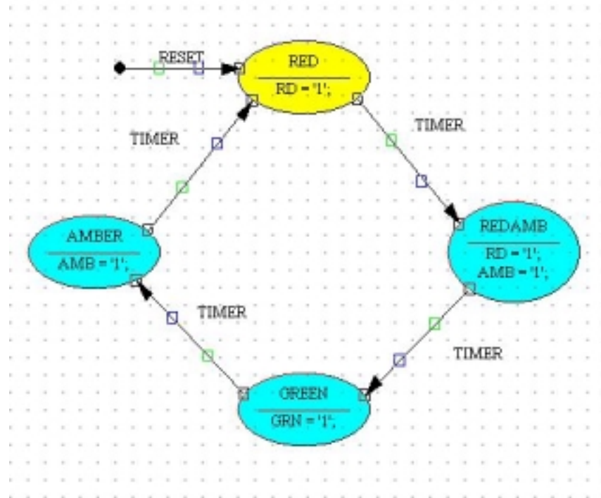
Figure 4.4.5 State Diagram
