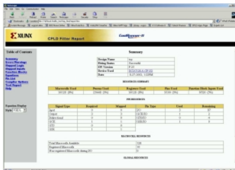
Fig 6.4.2 CPLD HTML Fitter Report
